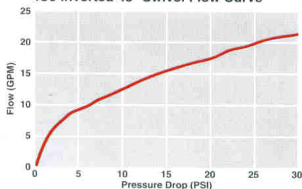
IC3 Inverted 45° Swivel Flow Curve
